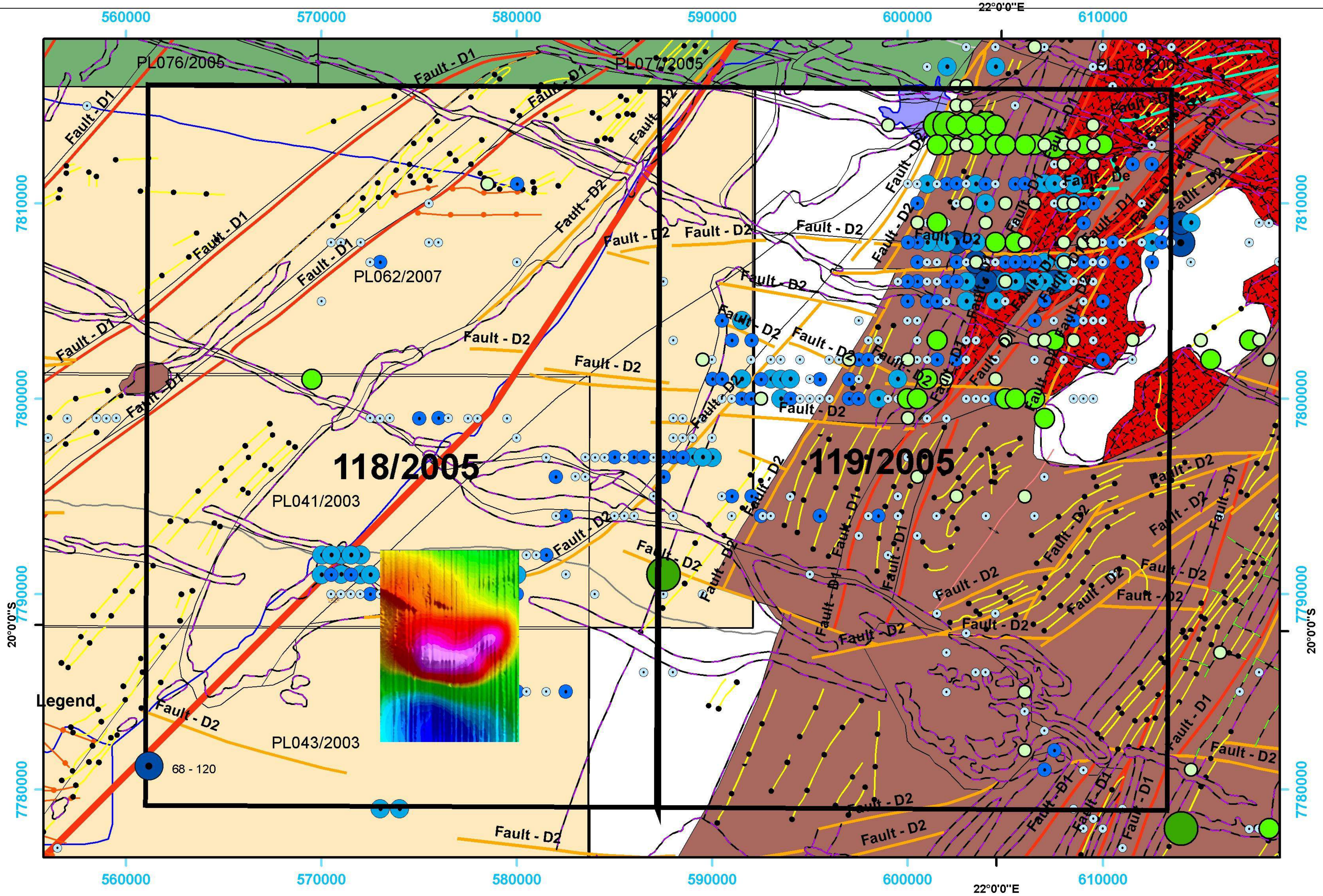
Map of Cu & Ni values ,faults and lineaments relative to other licenses. Also shown current area of surveying.
